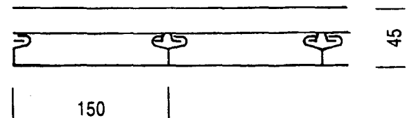
MK-P-T-PP-150, modul 150
