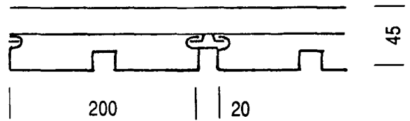
MK-P-T-D-100, modul 100/200
