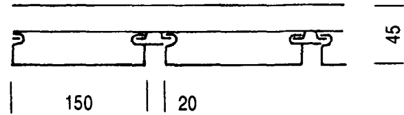
MK-P-T-SP-150, modul 150
